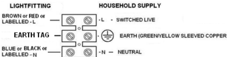
Wiring Details
